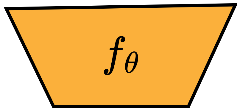
Embedding model
